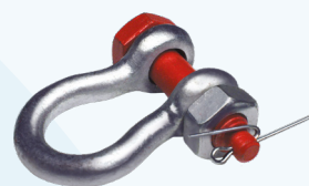
Bow Shackle Heavy-Duty with Nut Available from 5 mm to 19 mm W.L.L.: up to 4.750 Kg
